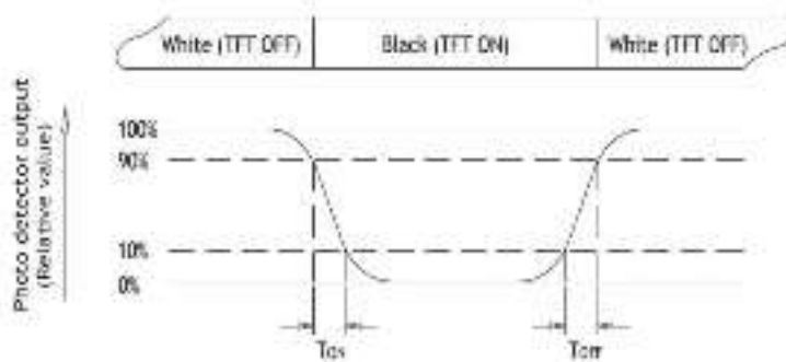
Fig. 6-3 Definition of response time
